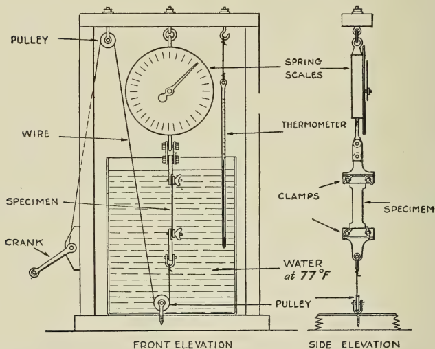
FIG. 202.—Instrument for Testing the Tensile Strength of Prepared Roofings.
